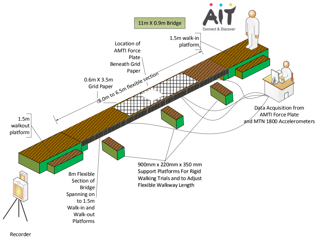
Figure 5: Schematic representation of trial set-up (not to scale)
