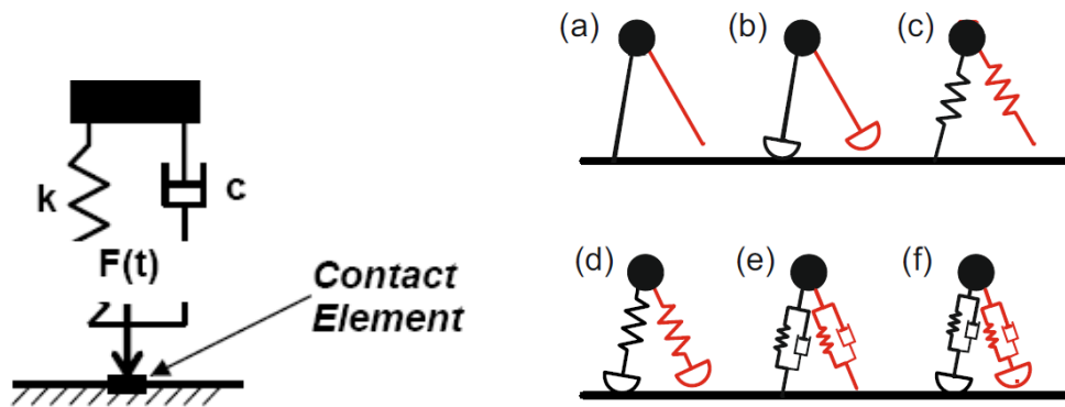
(a) Spring Mass Damper Model
