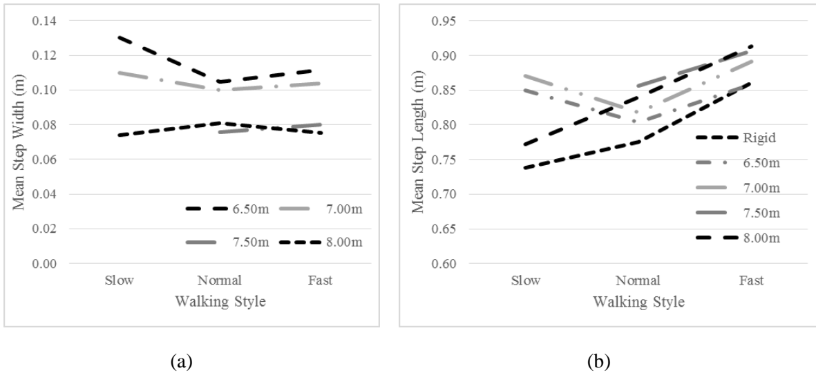
Figure 7. Mean Step Width (a) and Mean Step Length (b) Versus Walking Style for each bridge span
