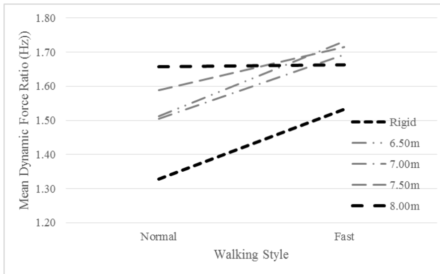
Figure 9. Mean Dynamic Force Ratio (DFR) versus Walking Style
