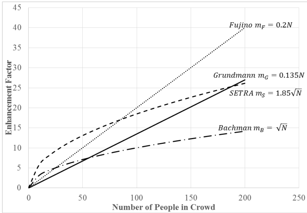
Figure 1 – Proposed Enhancement Factors for Vertical Loading Due to Crowd Synchronisation
