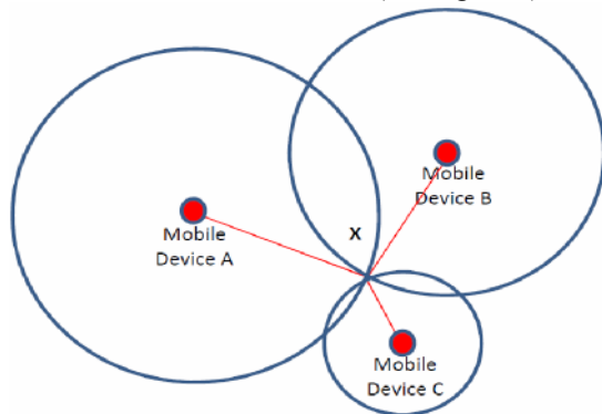
Figure 3: Trilateration example
